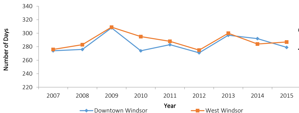
Figure 1.2 - Number of Good or Very Good Air Quality Index Days prior to AQHI Reporting
