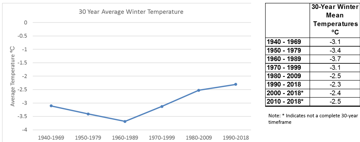
Figure 1: Historical Winter Mean Temperatures as Reported at Windsor Airport (Government of Canada)
