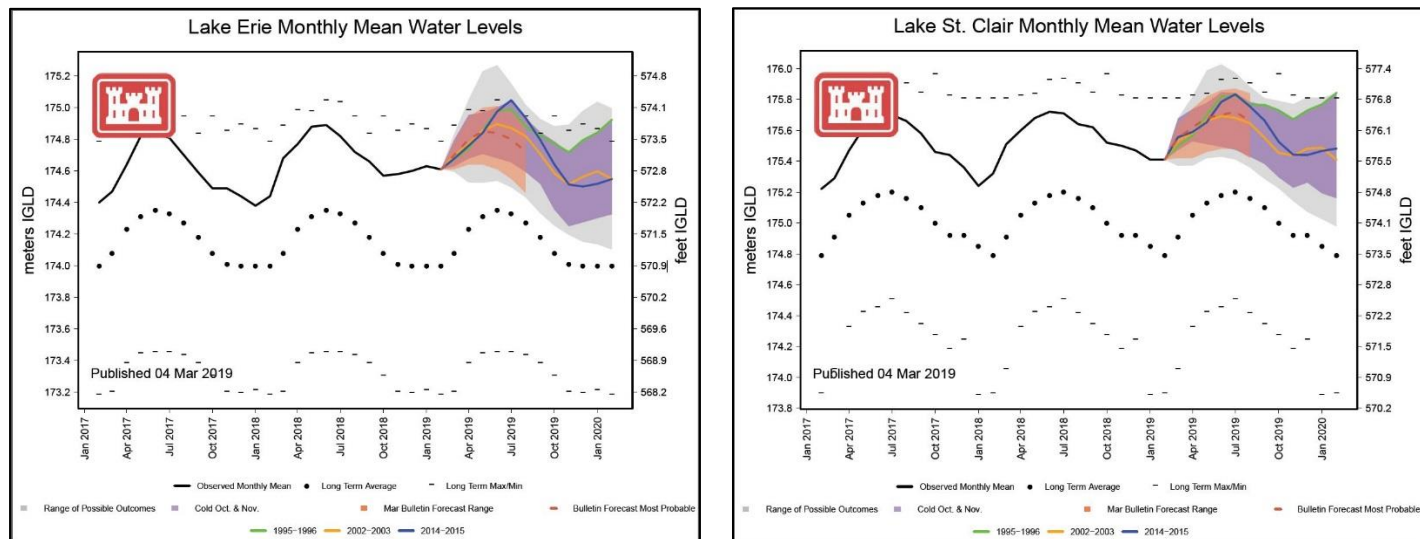
Figure 2: Short-term Lake Erie and Lake St. Clair Forecast (US Army Corps of Engineers)
