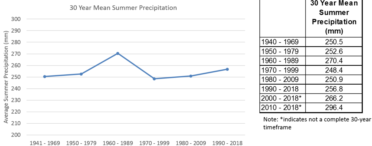
Figure 2: Historical Mean Summer Precipitation (Government of Canada)
