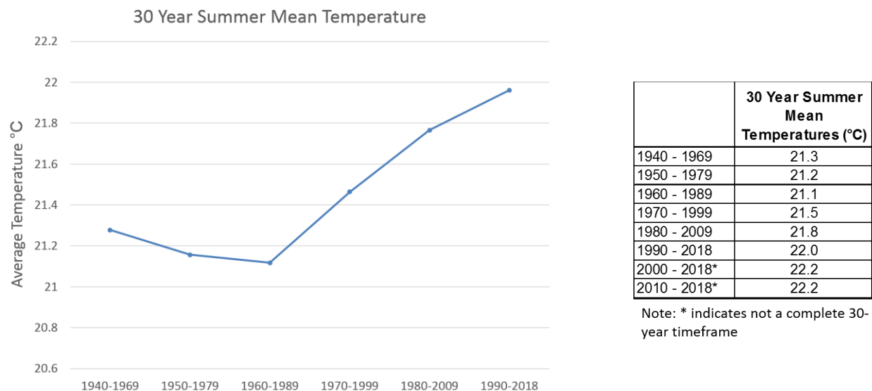
Figure 1: Historical Summer Mean Temperatures as Reported at Windsor Airport (Government of Canada)
