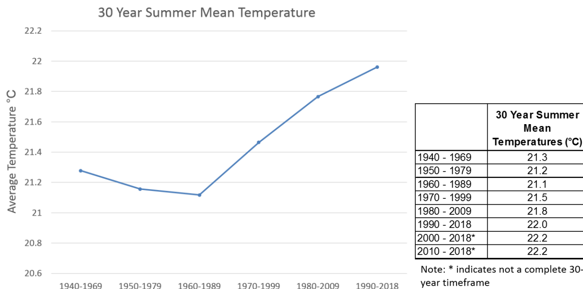
Figure 1: Historical Mean Summer Temperatures (Government of Canada)
