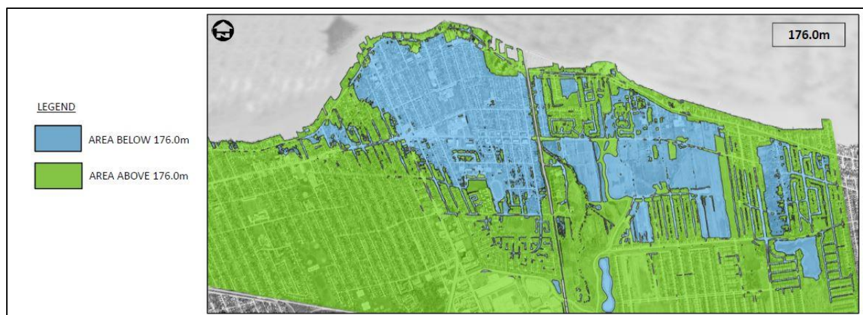
Figure 4: Area at Risk for Overland Flooding at current high water level of 176.0 m (Landmark Engineers, 2019)
