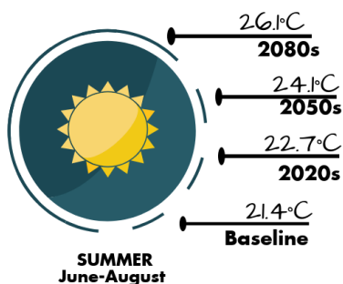
Figure 2: Summer Mean Temperatures Projections (ICLEI, 2018)
