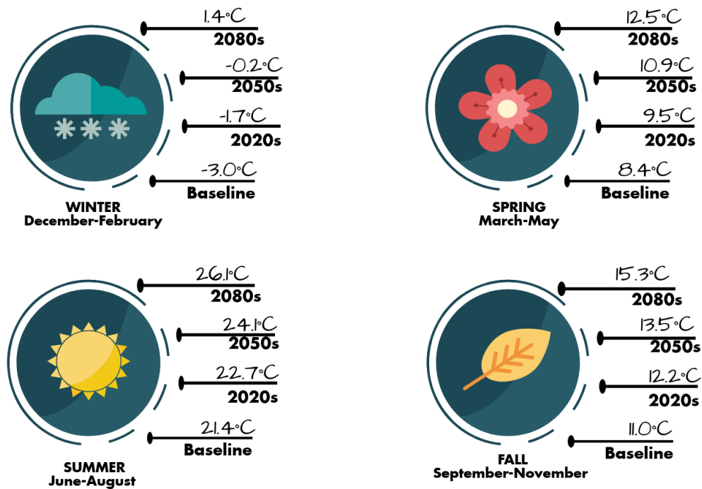
Figure 3: Annual Seasonal Mean Temperature Projections (ICLEI, 2018)
