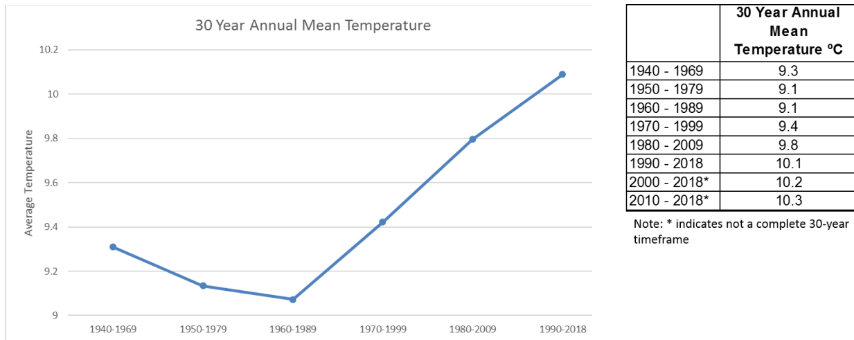
Figure 1: Historical Annual Mean Temperatures as Reported at Windsor Airport (Source: Government of Canada)
